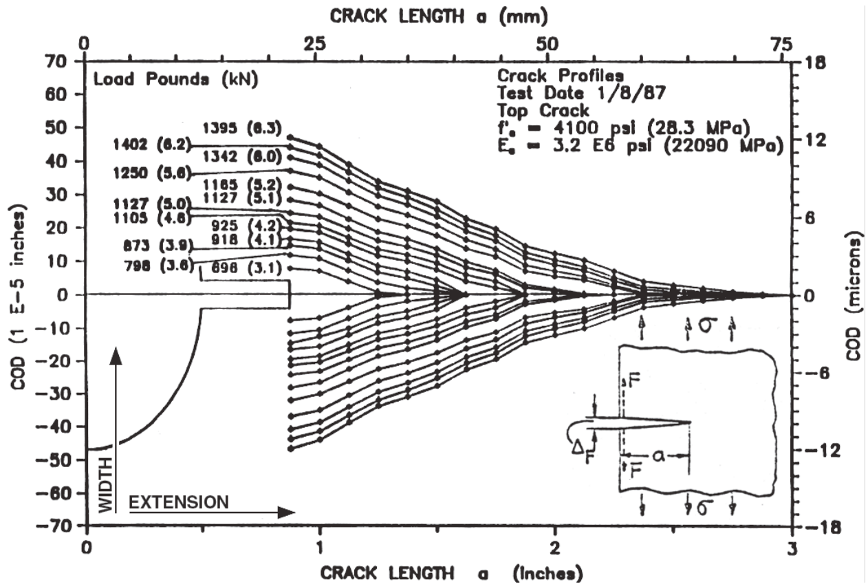
Figure 1 -Experimental observation that cracks extend as their width increases forms the foundation of fracture mechanics as well as the ACM measurement approach. Special visualization techniques were employed to measure the extension of a crack (marked by the rightward extension of the ">") as its width (COD or "crack opening displacement") increases (marked by the increasing width of the mouth of the ">" on the left. (Miller, 1989).
