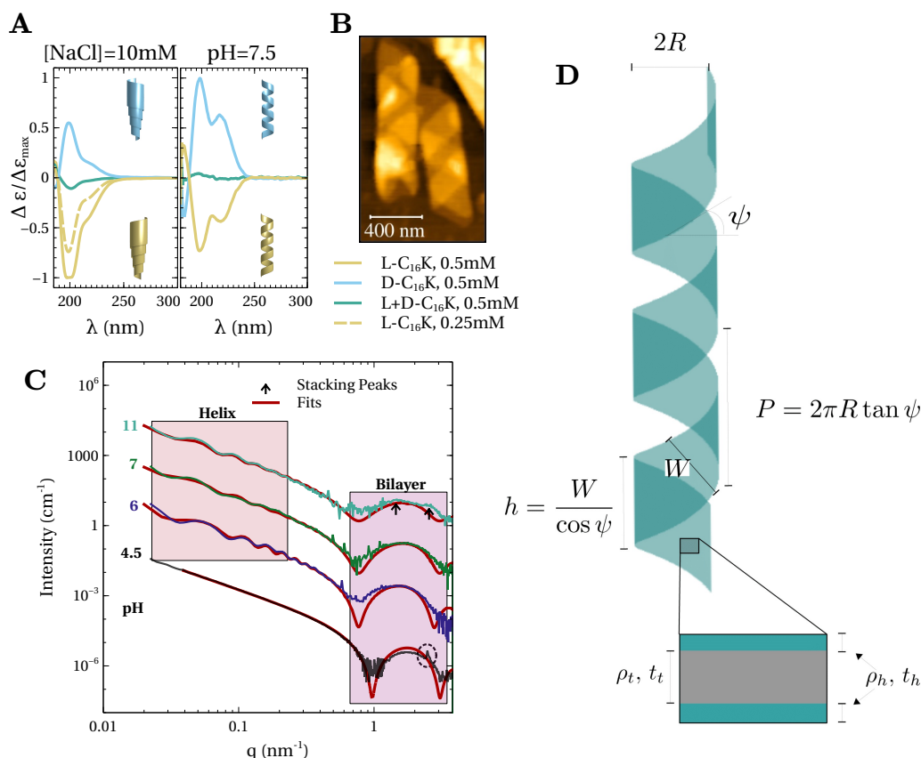
Figure 2.3: A. Circular dichroism spectra for C_{16}K_1 molecular assemblies in solutions with (1) pH \sim pK_a (right) and (2) 10 mM NaCl and pH \ll pK_a (left). Insets show schematics of the chiral shapes derived from cryo-TEM or AFM measurements. B. Ex situ AFM image of C_{16}K_1 assemblies at pH \sim 8.5 that were drop-cast and dried on a Si (1 0 0) substrate. C. In situ SAXS intensity profiles for 4 mM L- C_{16}K_1 assemblies in solutions at 4 different pH. The data for pH 6, 7, and 11 are scaled for clarity. Also shown are fits (red line) based on a planar bilayer ( pH = 4.5 ) or helix ( pH=6, 7, 11 ) models. D. Schematics of the helix model used to fit data. Left side shows a bilayer membrane that is twisted into a helix parametrized by three independent parameters. For example, the radius ( R ), the helix angle ( \psi ), and the width ( W ). Right side shows a cross-section of the bilayer membrane.
