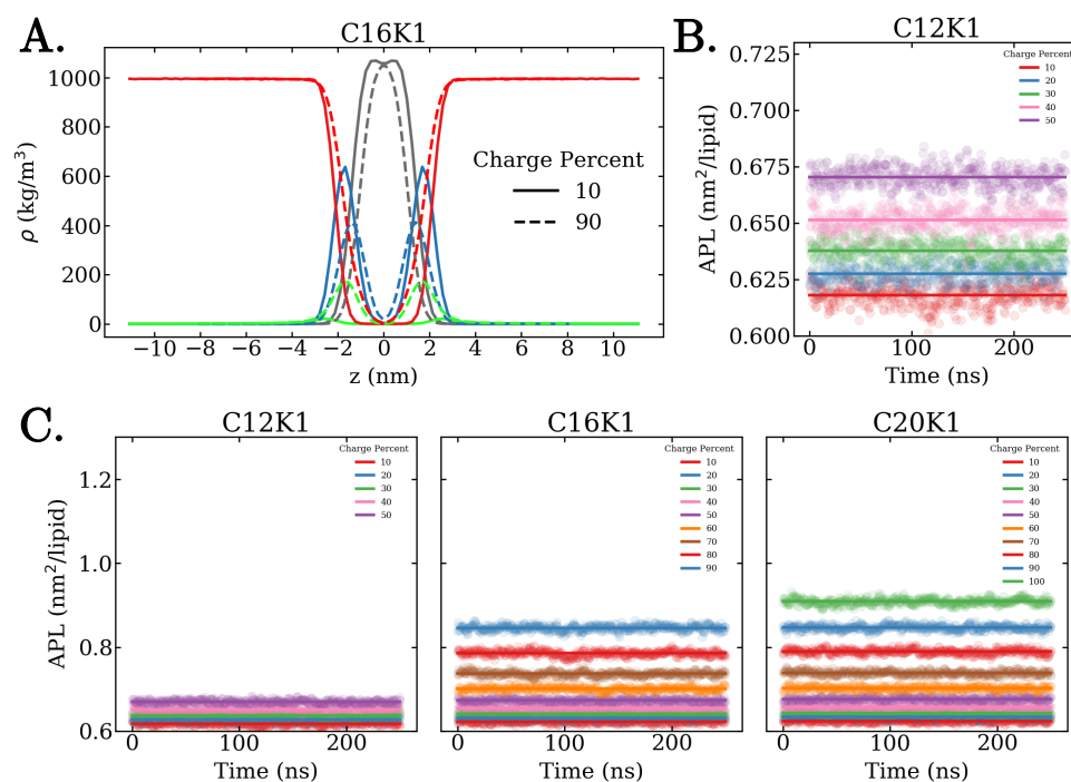
Figure 3.7: A. C 16 K 1 density plot for 10% and 90% charged bilayers. Excess water density (red) is found within the headgroup density peaks (blue) at larger charge percents. Tail region (gray) plateau is absent at higher charge percents and is replaced by a peak. Counterion density (green) are increased for larger charge percents to maintain electroneutrality. B. Area per lipid (APL) increases with increasing charge percent for C 12 K 1 bilayers. C. The effect is more pronounced for C 16 K 1 and C 20 K 1 , where all APL measurements are shown to scale for comparison across tail length. There is no recognizable change in area per lipid between tail lengths of stable bilayer simulations.
