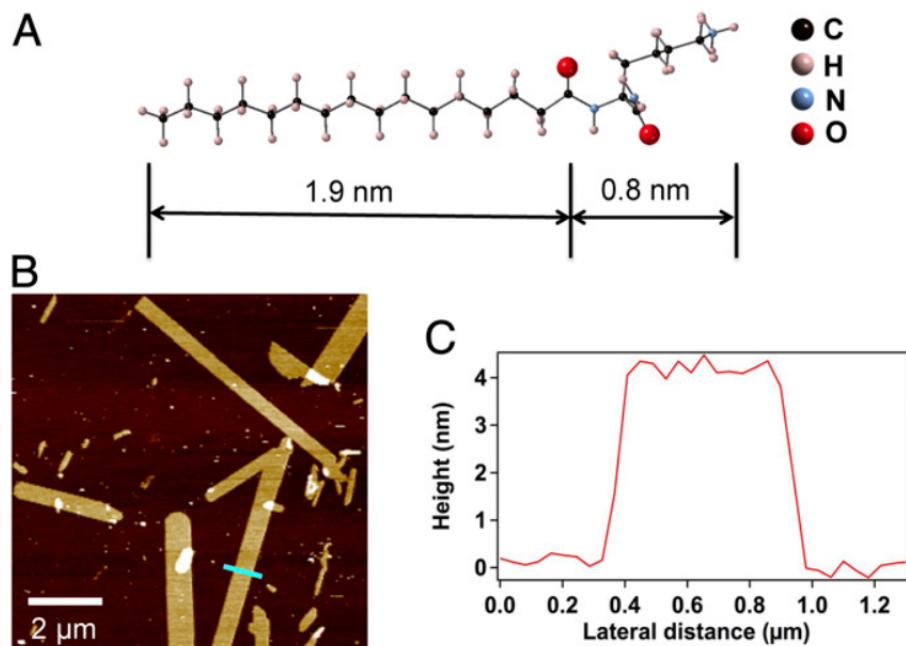
Figure 1.1: A. Molecular structure of +1 charged C 16 K 1 with estimates for hydrophobic tail and hydrophilic headgroup lengths. The molecular conformation was derived from an MD simulation for a single C 16 K 1 in water using the universal force field [65]. B. AFM image from a silica/water interface showing high aspect ratio C 16 K 1 nanoribbons. C. The height profile across a C 16 K 1 ribbon (green line in B ).
