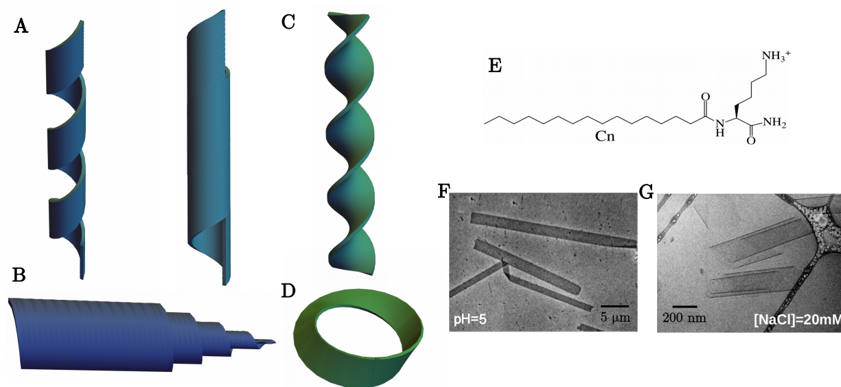
Figure 2.1: Schematics of chiral shapes: A. helical ribbon and closed helical tubule, B. cochleate (scroll-like), C. twisted ribbon, and D. möbius strip. E. Schematic for the molecular design for the homologous series of amphiphiles C_nK_1 . F. TEM image of L-C_{16}K_1 flat ribbons and G. cryo- TEM cochleate structure for L-C_{16}K_1 in [NaCl] = 20 mM. F. Credit to Changrui Gao, G. Credit to Erik W. Roth
